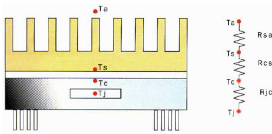
Figure 1: Thermal resistance circuit
