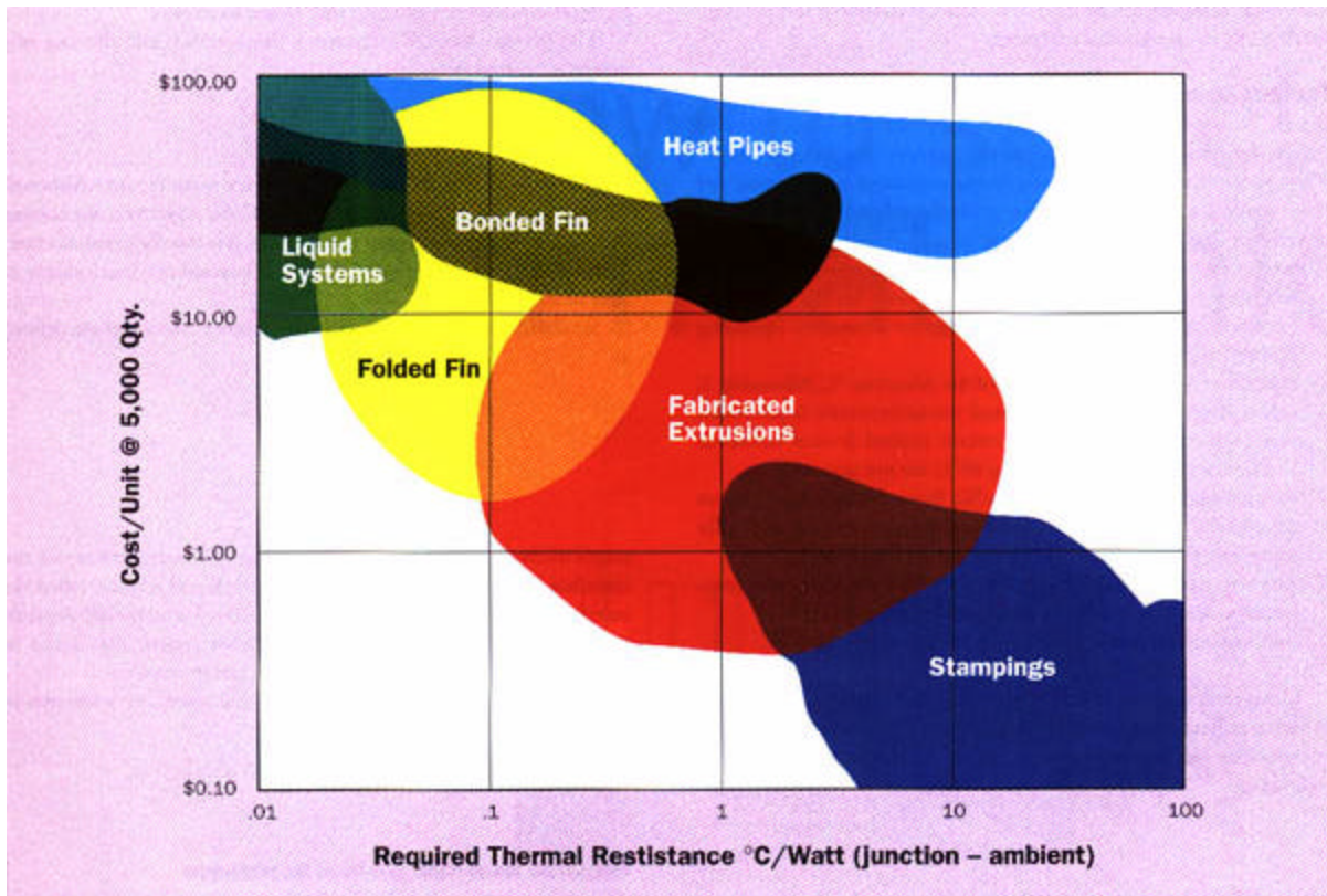
Figure 2: Cost versus required thermal resistance
