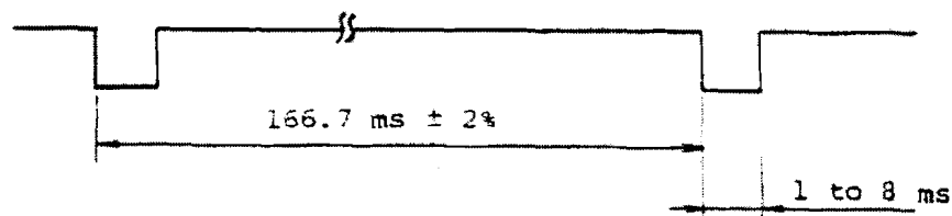
Fig. 3-4 Index Timing
