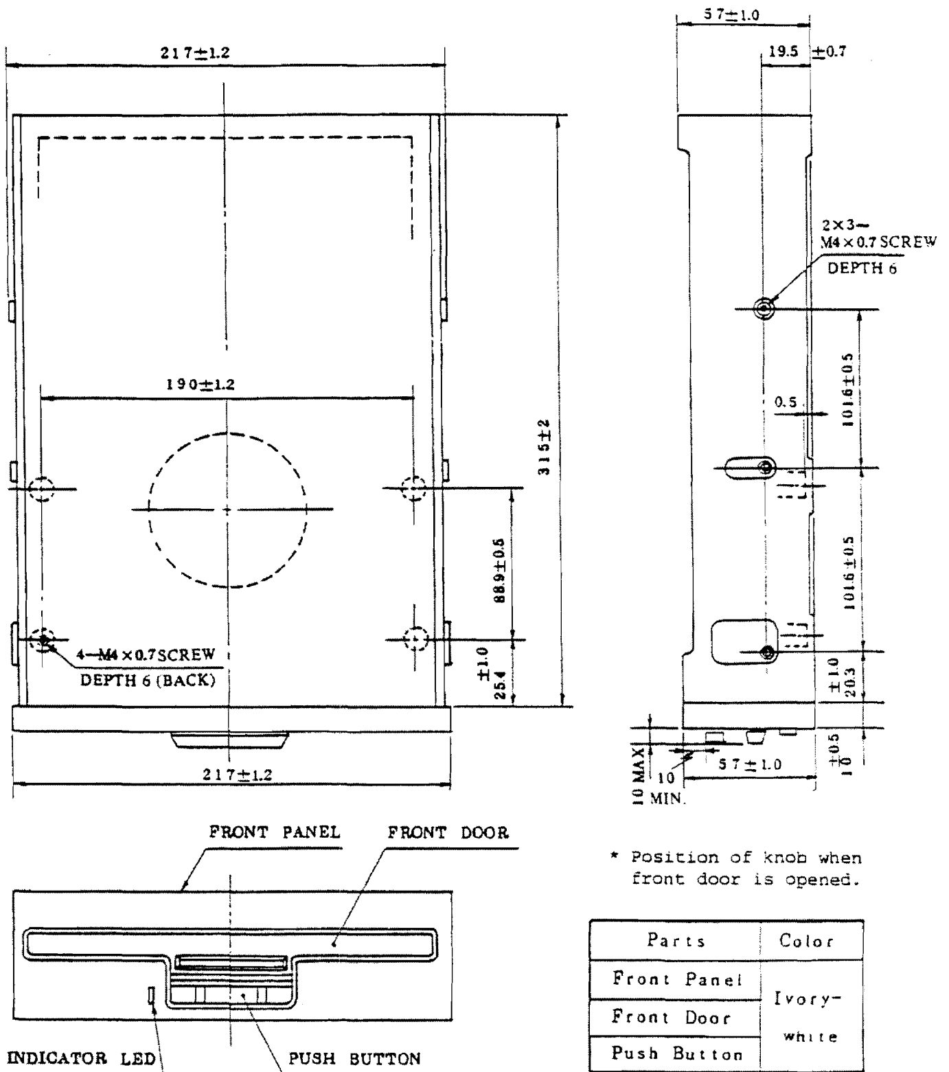
Fig. 7-1 M2896 Drive Dimensions
