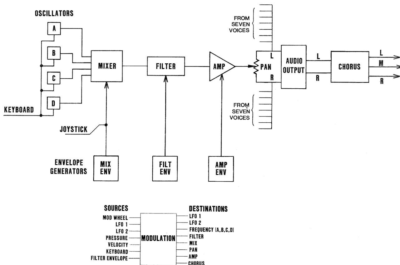
Figure 6.1 General Block Diagram
