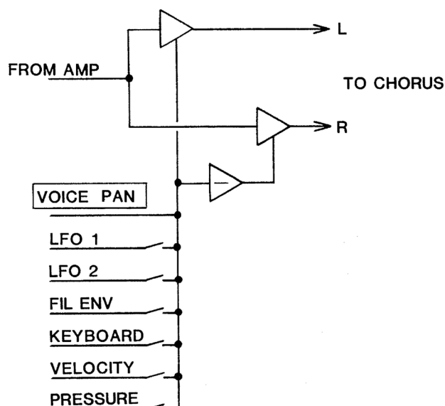
Figure 11-1 PAN MODULE
