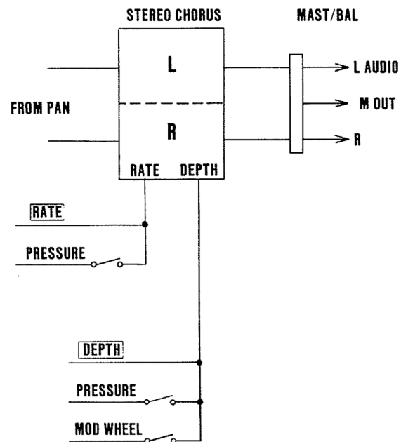
Figure 12-1 CHORUS MODULE
