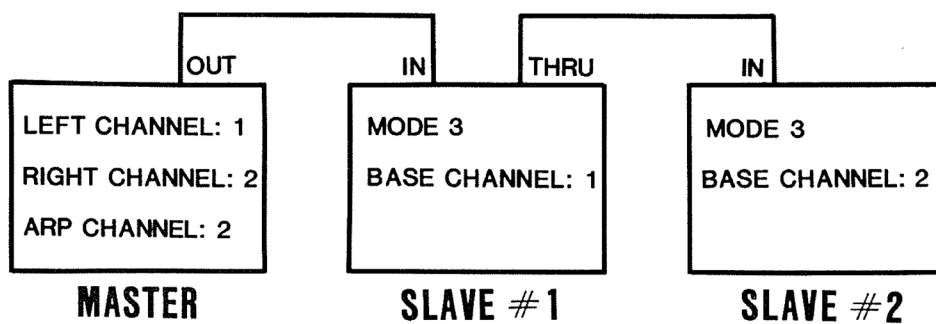
Figure 14-3 MULTI-CHANNEL OPERATION
