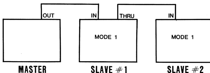
Figure 14-1 BASIC MIDI CONNECTIONS
