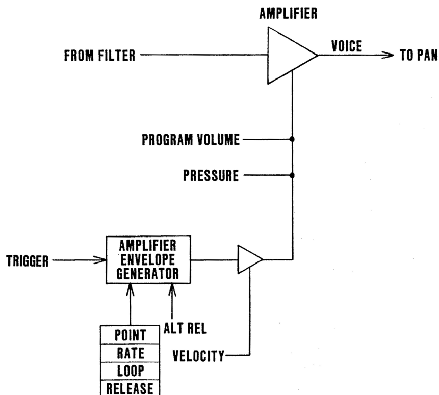
Figure 8-6 AMPLIFIER MODULE
