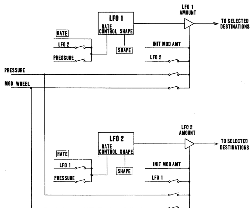
Figure 9-1 LFO MODULE
