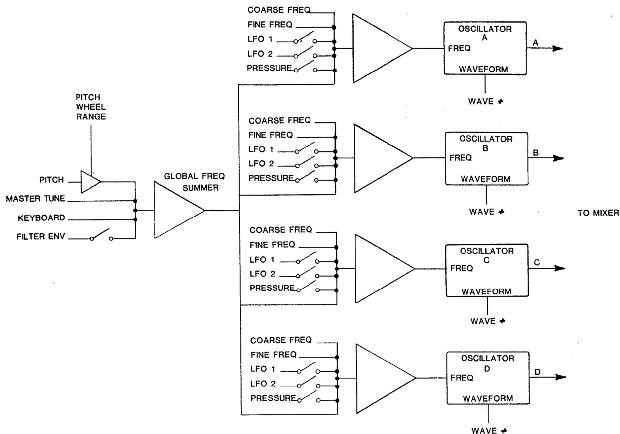
Figure 6-2 OSCILLATOR FREQUENCY CONTROL
